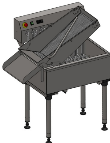
Drain position
