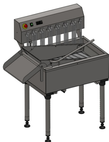
Work position
